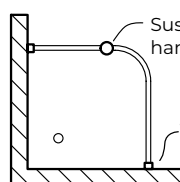
L-shaped (shower)
